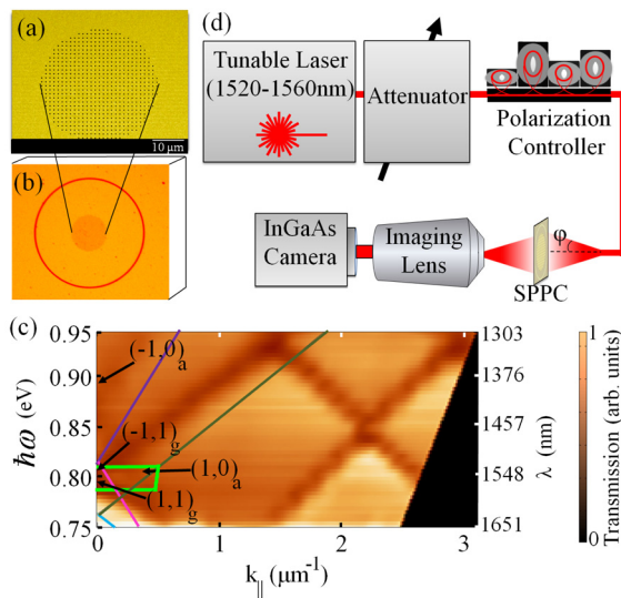
FIG. 1. (Color online) (a) SEM image of the SPPC and (b) optical microscope image of the SPPC surrounded by a scattering ring. (c) Measured SPPC transmission dispersion (2D map) and (lines) eigenmode positions estimated from Eq. (1); notations “a” and “g” correspond to the modes of air-Au and glass-Au interfaces, respectively. (d) Experimental arrangement for characterization of the SPPC wavelength and polarization dispersive properties.
